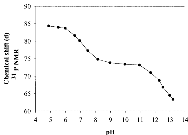
Figure 4. Determination of pK a values of BPi; plot of BPi's 31 P NMR chemical shift in H 2 O as a function of the pH; two inflection points are observed in the pH range 4.87–13.20
