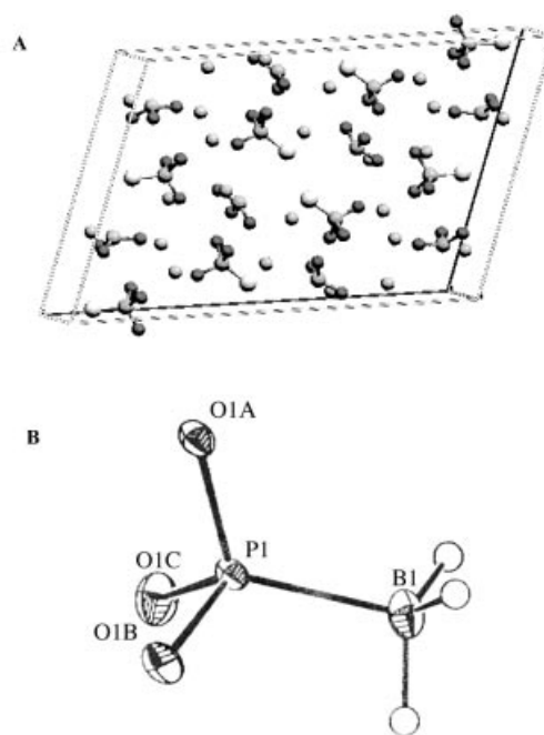
Figure 2. X-ray crystal structure of BPI: A) unit cell includes eight BPI molecules, eight H-phosphonate molecules, and 24 ammonium ions; hydrogen atoms are omitted to clarify the BPI geometry; B) ORTEP drawing of BPI; crystal data of 2a : monoclinic, P2_1/c ; a = 23.616(5) Å, b = 6.3470(13) Å, c = 15.325(3) Å; V = 2172.9(8) Å 3 ; Z = 12 ; D_{\text{calcd.}} = 1.623 g/cm 3 ; F(000) = 1104 ; 3094 reflections collected, R = 0.1015 , R_w = 0.2345 , GOF = 1.286; selected bond lengths [Å] and angles [°]: P(1)–O(1A) 1.524(7), P(1)–O(1B) 1.617(7), P(1)–O(1C) 1.583(7), P(1)–B(1) 1.891(11); O(1A)–P(1)–O(1C) 104.0(4), O(1A)–P(1)–O(1B) 105.3(4), O(1C)–P(1)–O(1B) 104.4(4), O(1A)–P(1)–B(1) 118.2(5), O(1C)–P(1)–B(1) 113.0(5), O(1B)–P(1)–B(1) 110.7(5)
