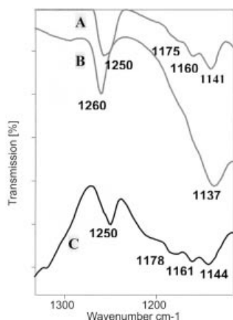
Figure 3. IR spectra of BPi 2c (germanium cell; 1300–1100 cm −1 ; cutoff: 680 cm −1 ): A) methanolic solution; B) aqueous solution; C) neat sample
