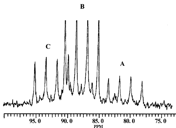
Figure 5. ^{31}\text{P} NMR spectrum of BPi 2b in methanolic solution
